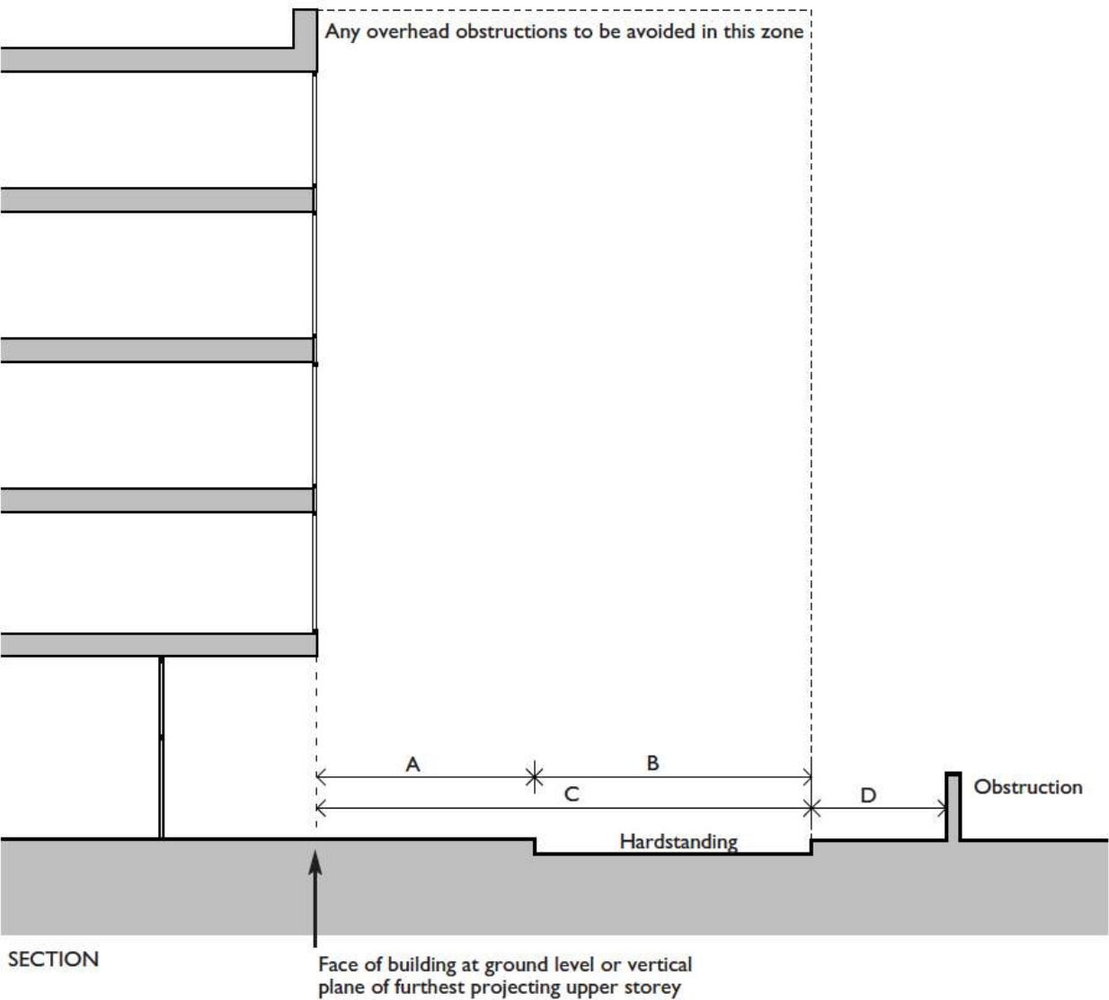
Diagram 32 Fire appliance (high reach) access to buildings
