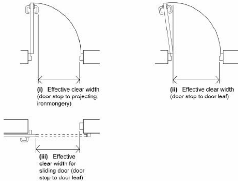
Diagram 35 Corridors, Passageways and Internal Doors to Dwellings (Showing Measurement of Effective Clear Width)
