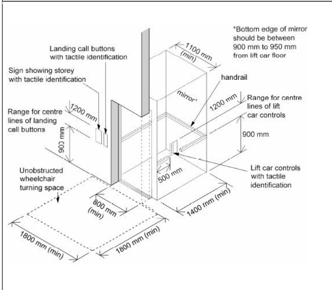
Diagram 13 Key Dimensions Associated With Passenger Lifts
