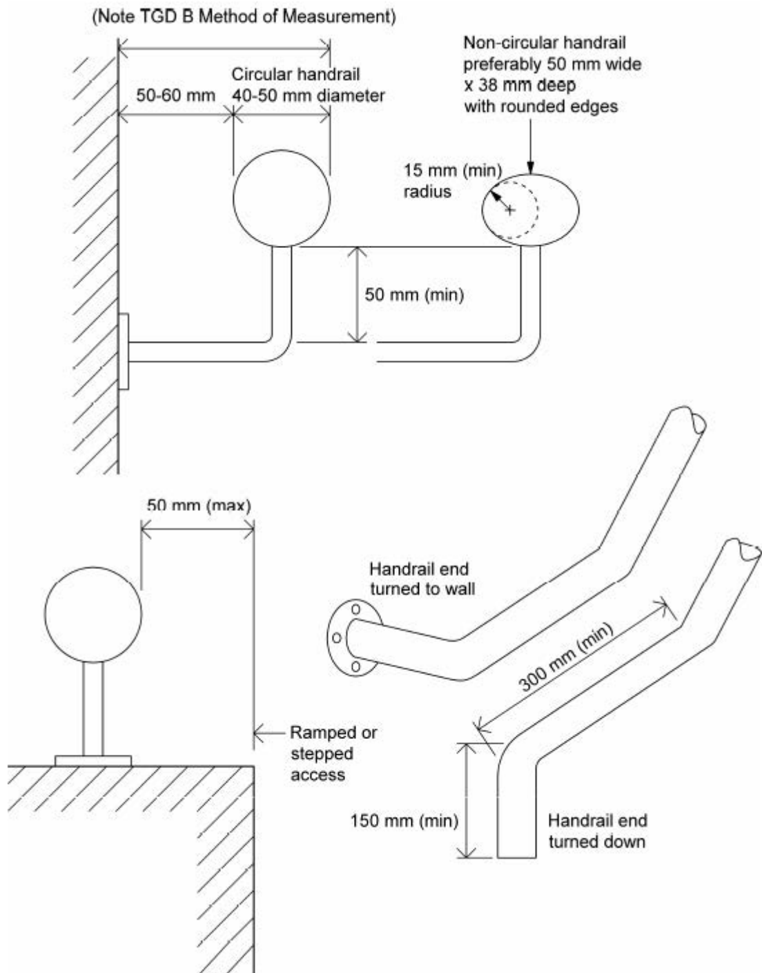
Diagram 7 Handrail Design
