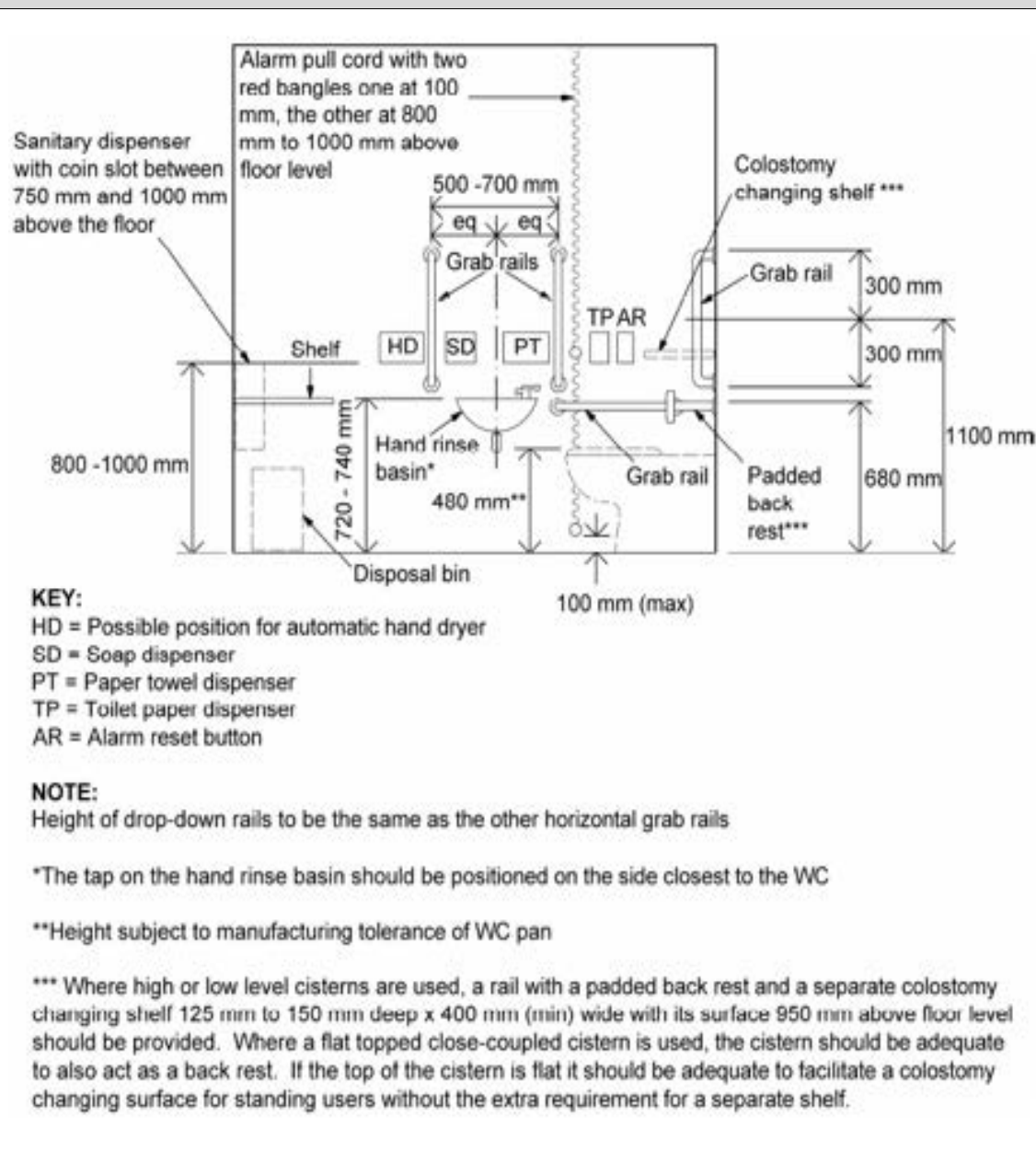
Diagram 16 Heights of Various Fittings on Wall A of A Wheelchair Accessible Unisex WC (Refer to Diagram 15a or 15b)
