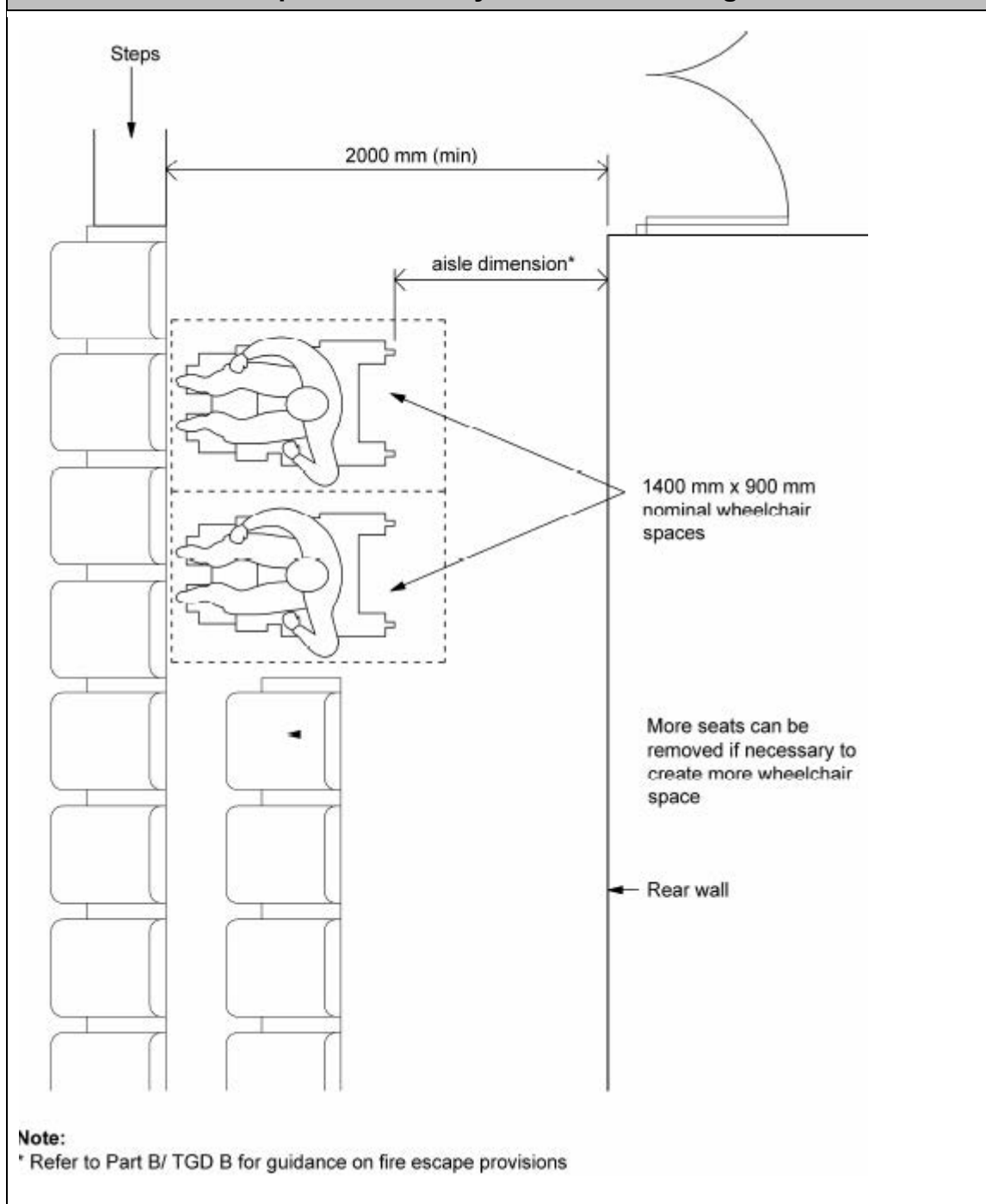
Diagram 29 An Example of Wheelchair Space Provision in an Audience and Spectator Facility with Fixed Seating
