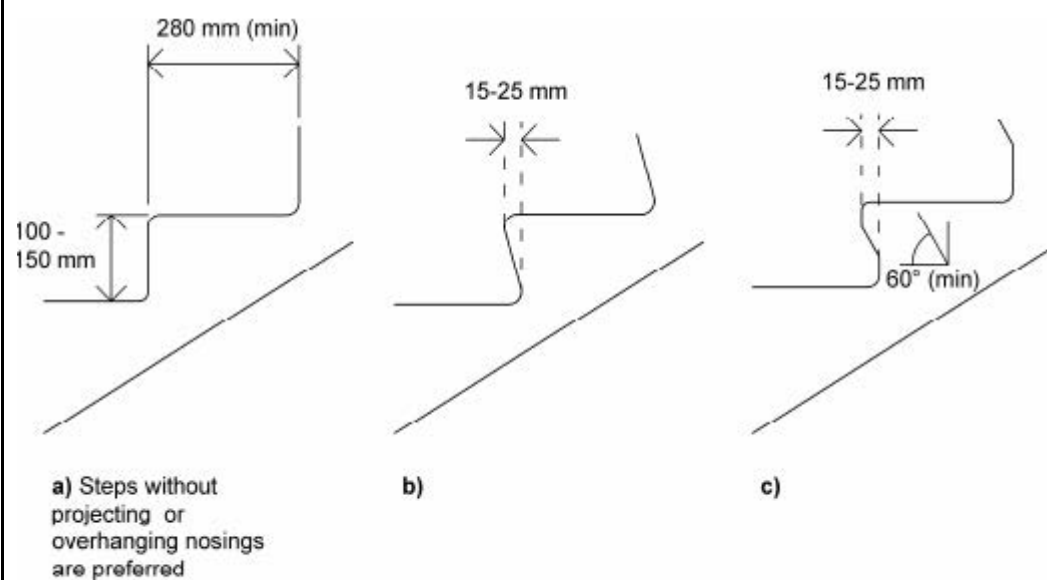
Diagram 34 Examples of External Step Profiles
