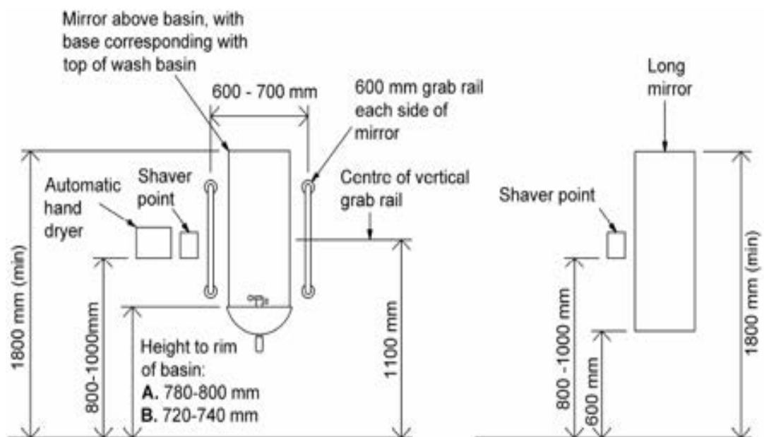
Diagram 17 Location of Independent Mirrors, Accessories and Washbasin
