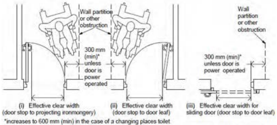
Diagram 10 Effective Clear Width and Visibility Requirements of Doors
