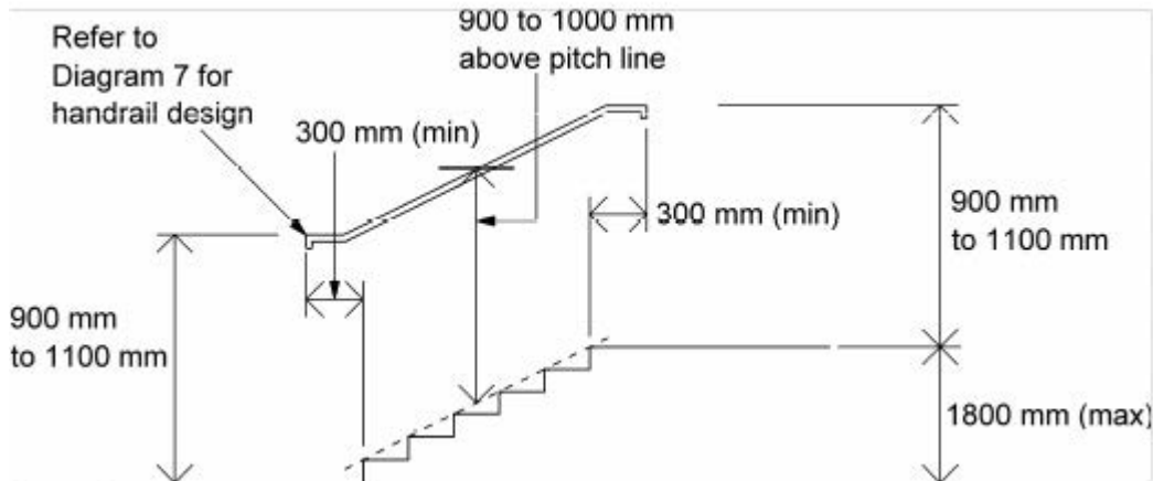
Diagram 14 Key Dimensions Associated with Internal Stairs Suitable for Ambulant Disabled People
