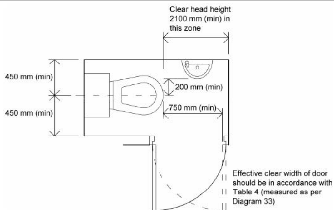
Diagram 37 Example of WC compartment for small dwellings
