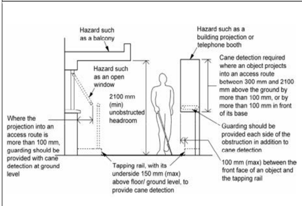
Diagram 2 Hazard Protection on Access Routes
