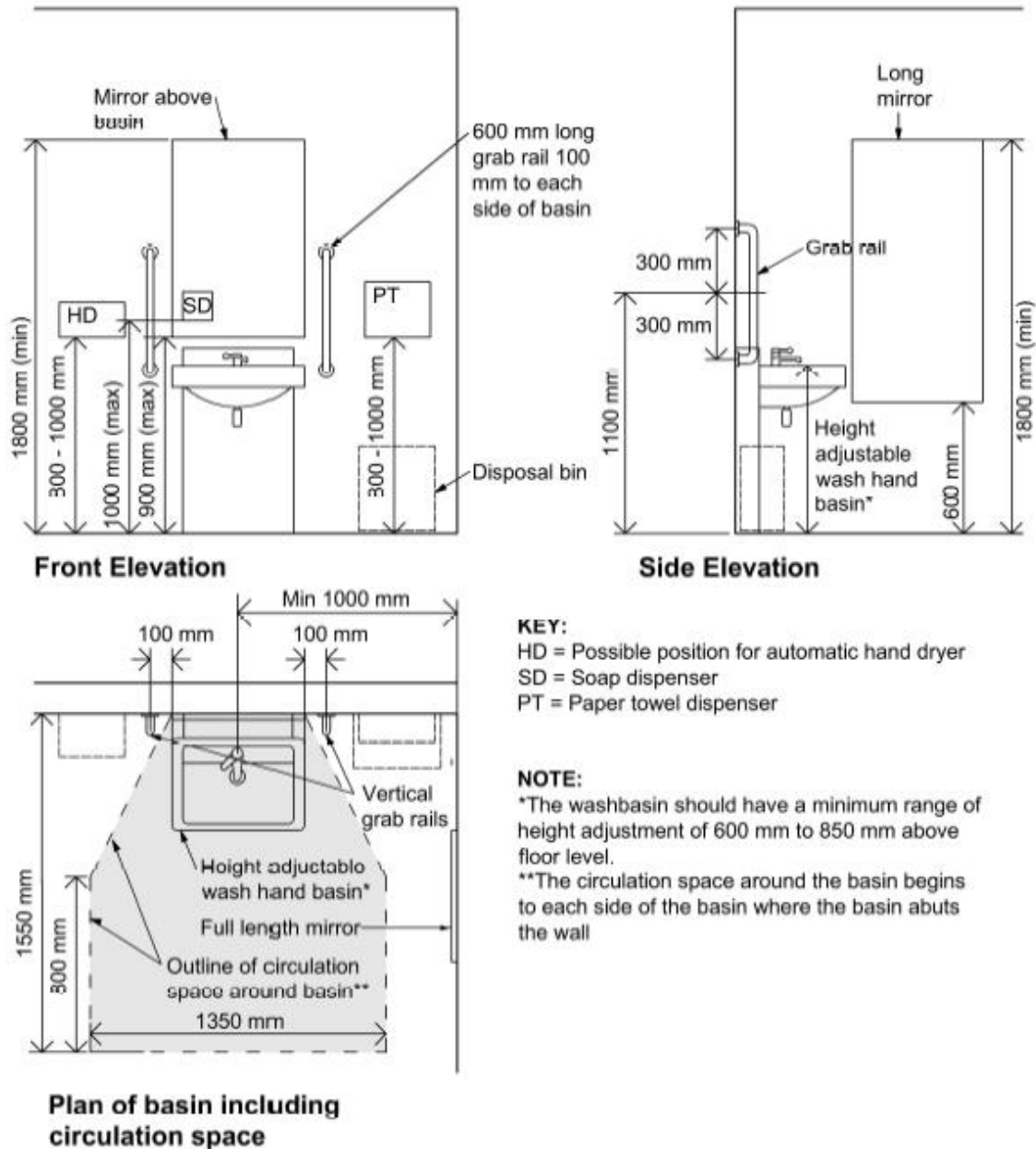
Diagram 27(b) Layout, Circulation Areas, Fixtures and Fittings for the Height Adjustable Wash Hand Basin
