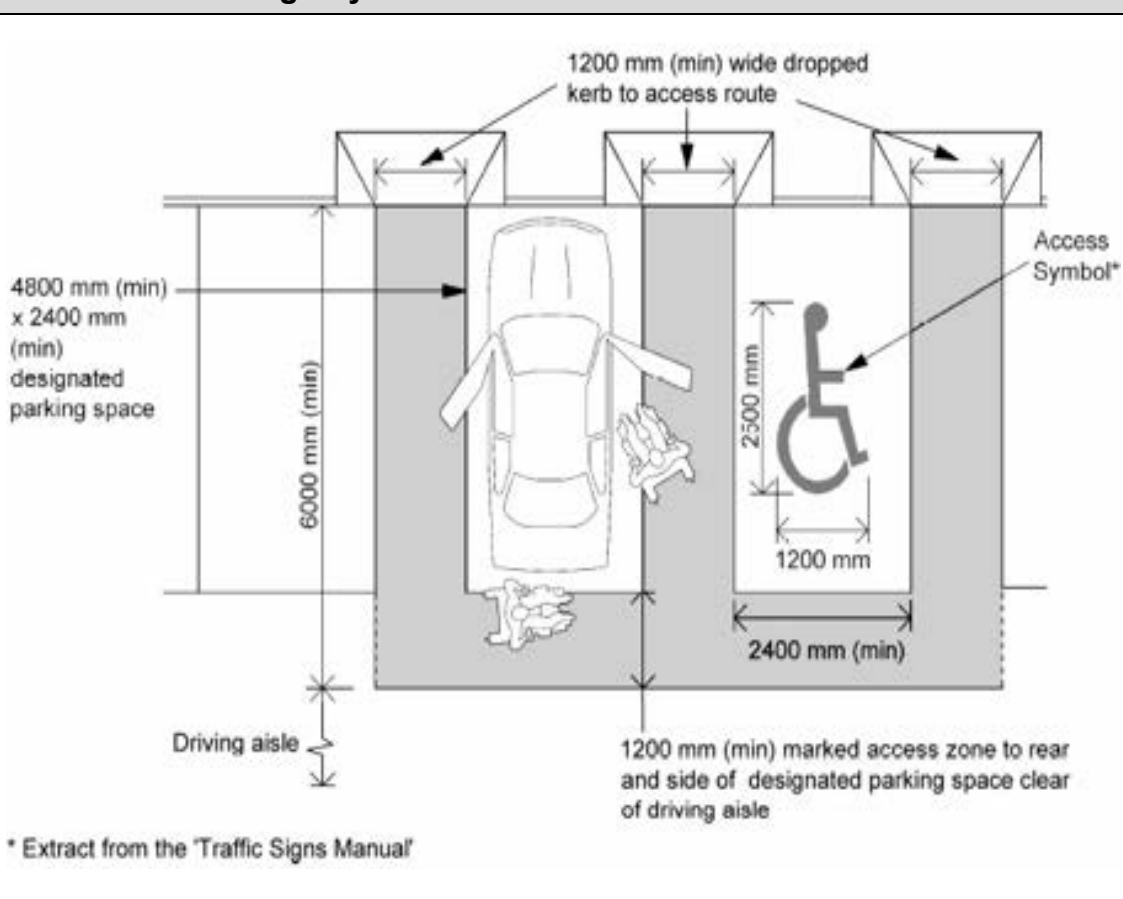
Diagram 8 Access Around Designated On-Site Perpendicular Parking Bay
