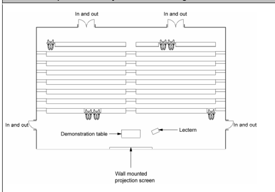
Diagram 28 An Example of Wheelchair Spaces in in Audience and Spectator Facility With Fixed Seating
