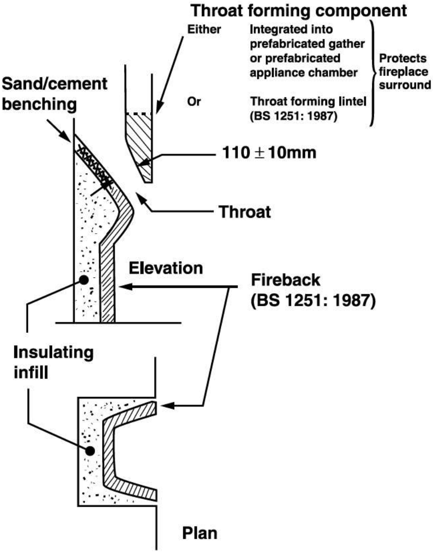
Diagram 29 Open fireplaces: throat and fireplace components
